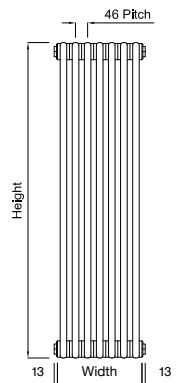
Forza Vertical Elevation
