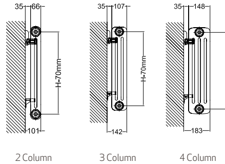
Forza Horizontal Section
