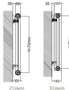
Forza Vertical Section
