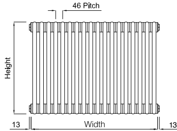
Forza Horizontal Elevation
