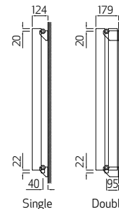
Adagio 70 Vertical Section
