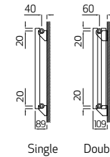
Adagio 35 Horizontal - Single and Double Section
